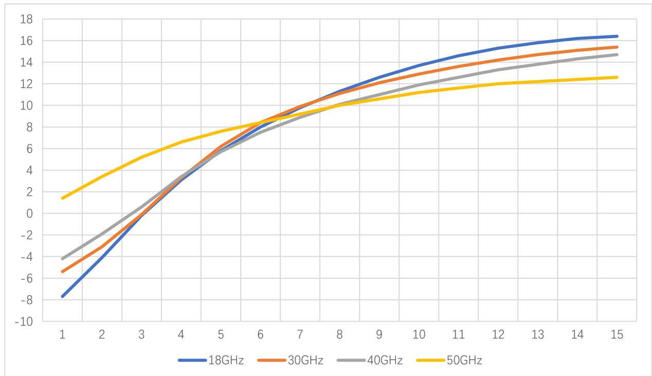
Pout vs Pin at 18/30/40/50GHz
